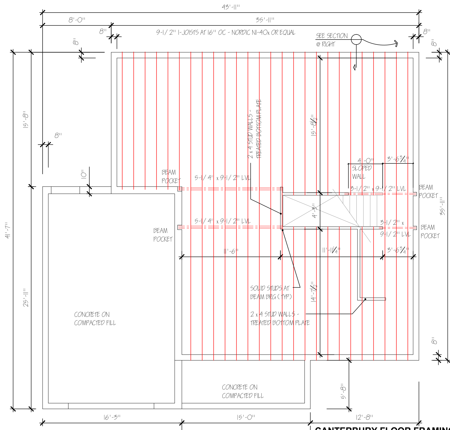
CANTERBURY FLOOR FRAMING SCALE: \frac{3}{16}" = 1'-0"
